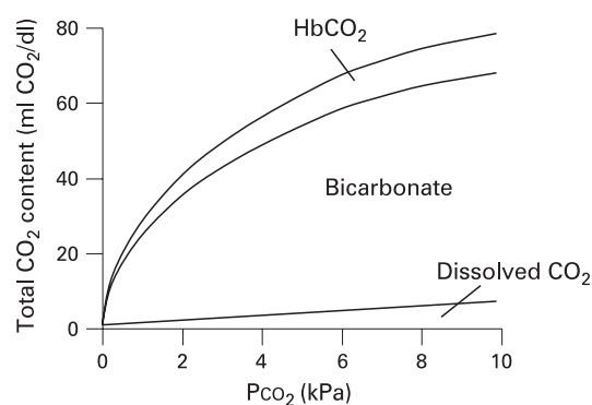
Figure 6 Total carbon dioxide dissociation curve. PCO_2 , carbon dioxide tension; HbCO_2 , carbamino haemoglobin.
