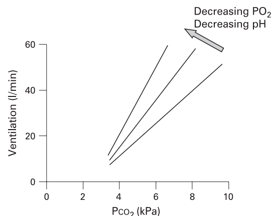
Figure 7 Effect of arterial carbon dioxide tension ( PA_{CO_2} ) on ventilation with interaction of acidosis and hypoxaemia.
